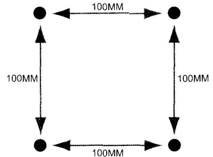
VESA 100 Fittings
