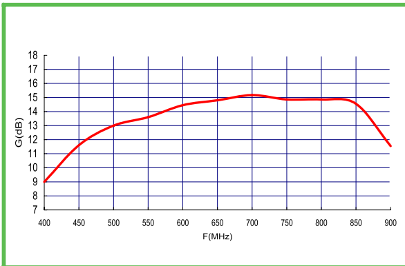
Aerial Gain
