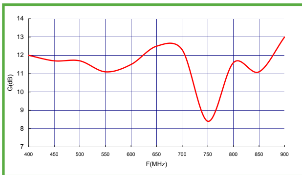
Aerial Gain
